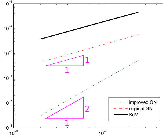
Figure 4: Convergence rate. Log-log plot of the normalized l^2 norm of the error as a function of c - 1 .
