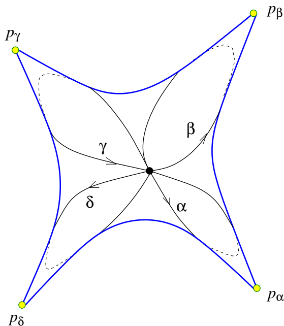
FIGURE 1. The four punctured sphere.
