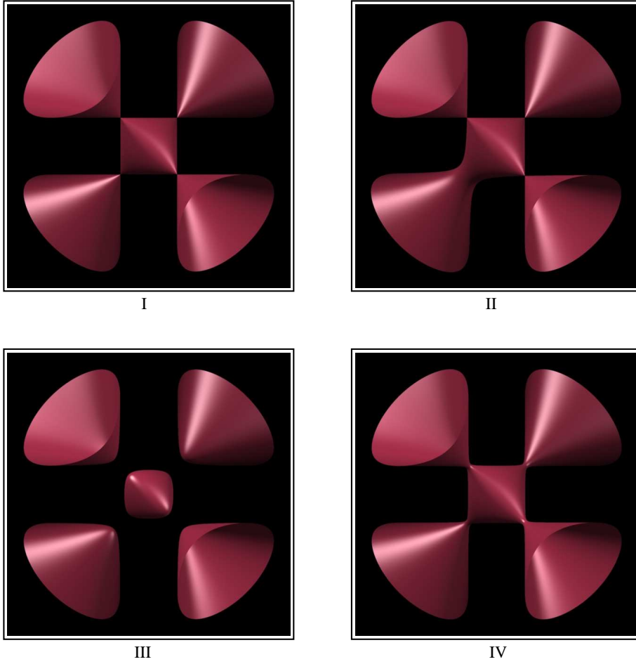
FIGURE 2. Four examples. I. The Cayley cubic S_C ; II. S_{(-0.2, -0.2, -0.2, 4.39)} ; III. S_{(0, 0, 0, 3)} ; IV. S_{(0, 0, 0, 4.1)} .
