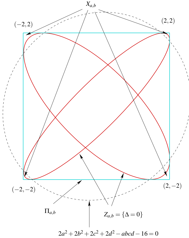
FIGURE 5. Z restricted to the slice \Pi_{a,b} .
