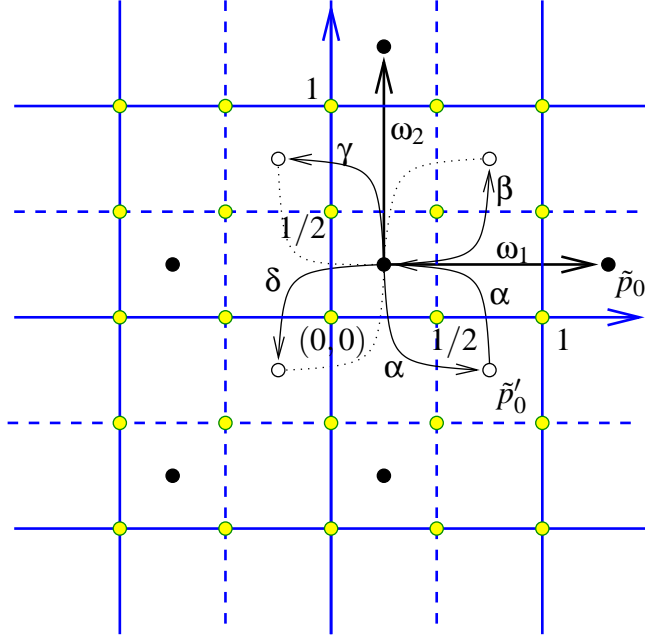
FIGURE 3. The torus cover.
