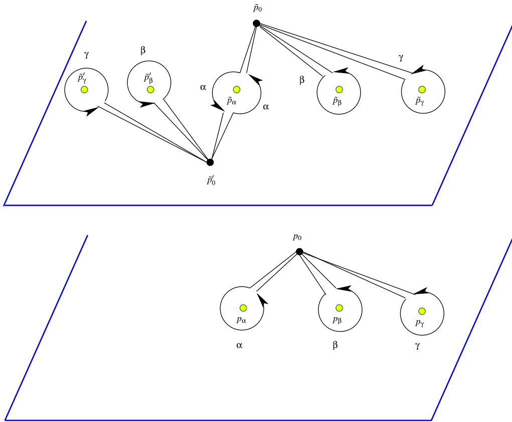
FIGURE 6. The two-fold cover. (the point p_\delta is at infinity)
