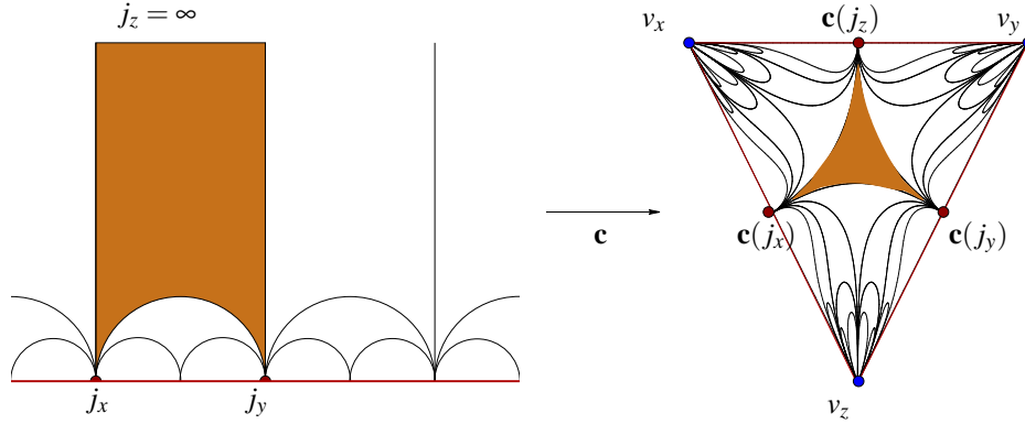
FIGURE 4. Conjugation for the Markov example. The right hand part of this figure depicts the dynamics of \Gamma_2^* on S_{M^+}(\mathbf{R}) , but viewed in \mathbb{P}^2(\mathbf{R}) after the birational change of variables [x : y : z : w] = [XQ : YQ : ZQ : XYZ] , with Q = X^2 + Y^2 + Z^2 . This change of variables sends the interior of the triangle \{X \geq 0, Y \geq 0, Z \geq 0\} onto S_{M^+}(\mathbf{R}) .
