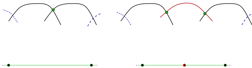
FIGURE 2. Blowing-up one point.
