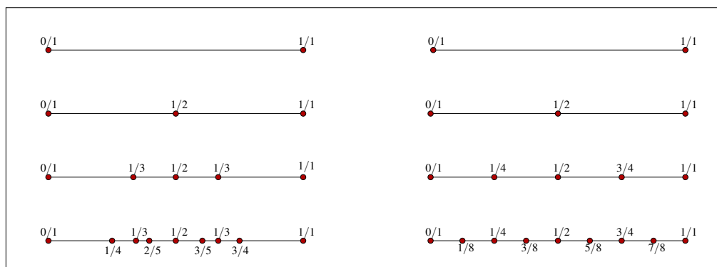
FIGURE 3. On the left, the Farey algorithm. On the right, the dyadic one. Here k = 0 (top), to k = 3 (bottom).
