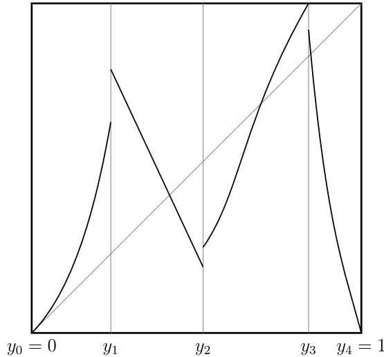
Fig. 1. The graph of a GPM map, with d = 4 .
