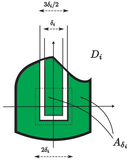
Figure 5.2: The set A_{\delta_i} := (D_i \cap \mathcal{S}_{\delta_i}) \cup (D_i \setminus \text{Int}(\mathcal{S}_{\frac{3\delta_i}{2}})) , on which \hat{\eta}_i is defined.
