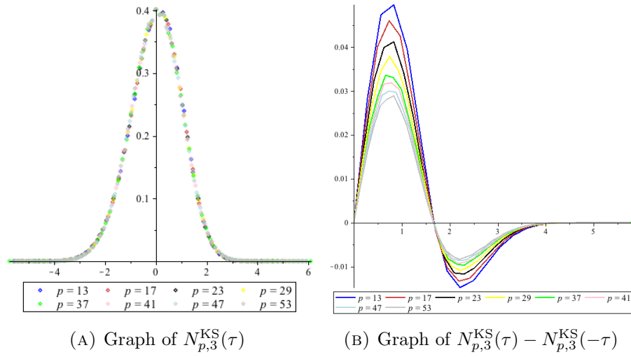
FIGURE 3. Trace distribution
