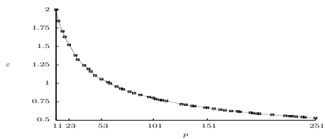
FIGURE 2. Overhead \varepsilon
