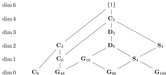
FIGURE 1. Automorphism groups
