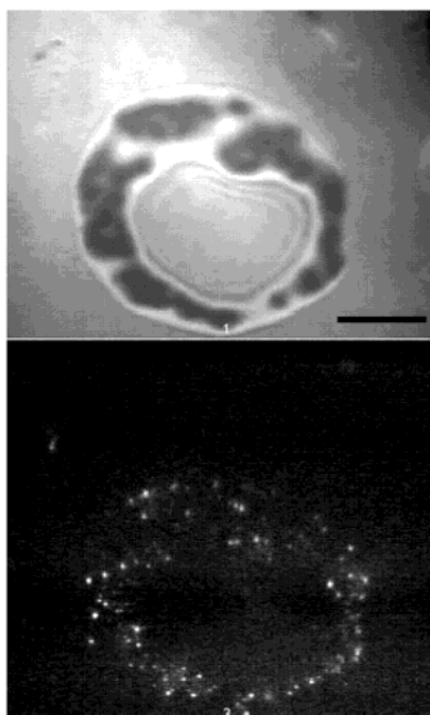
Figure 4. Typical image of a stably adhering vesicle containing RGD chalcone 5 (2 mol %) in matrix DMPC/Chol/DMPE-PEG 2000 (50:50:3) ( \alpha_{11b}\beta_3 integrin surface): (top) by RISM and (bottom) by fluorescence optical microscopy ( \lambda_{\text{exc}} = 450 ). The fluorescence image was obtained from accumulation of several recorded video images (one image every 40 ms during 500 ms) before the fast bleaching of the probe (around 100 ms). Notice that all the fluorescent spots are localized in the contact zone. The scale bar represents 10 \mu\text{m} .
