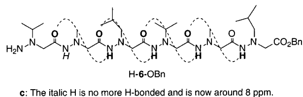
Figure 4. Nearest-neighbor hydrogen-bonding models for hexamers 6.
