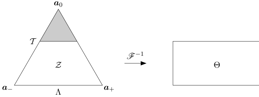
Figure 2: The homographic transformation from \mathcal{Z} onto \Theta
