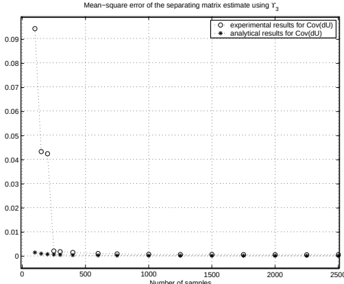
Fig. 3. Variance of estimated separating matrix \mathbf{U} obtained by maximization of \Upsilon_3(\mathbf{U}) .
