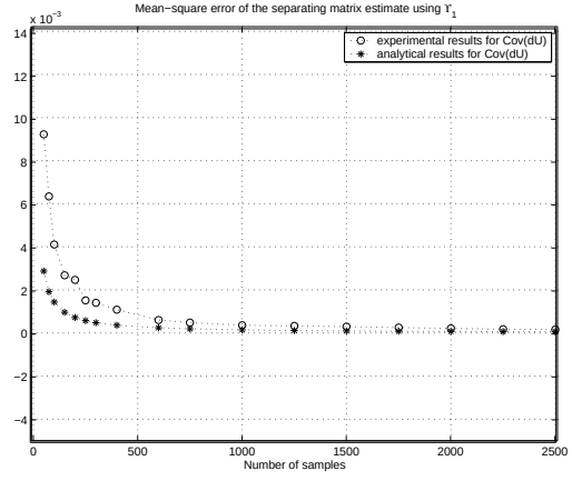
Fig. 1. Variance of estimated separating matrix \mathbf{U} obtained by maximization of \Upsilon_1(\mathbf{U}) .
