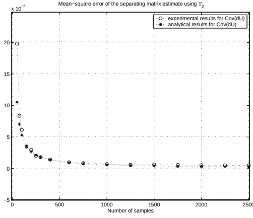
Fig. 2. Variance of estimated separating matrix \mathbf{U} obtained by maximization of \Upsilon_2(\mathbf{U}) .
