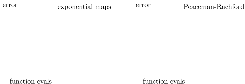
Figure 5: Plot: Nonlinear case – Error ( L^2 norm at time T ) versus number of evaluations of the basic method \Phi_h . Strang splitting (dotted lines), and “quadruple jump” composition method \Psi_h^{(4)} (solid line), extrapolation method (dashed-dotted line), extrapolation method (dashed lines). Left picture: Basic method is the Strang splitting with exponential maps. Right picture: Peaceman-Rachford formula.
