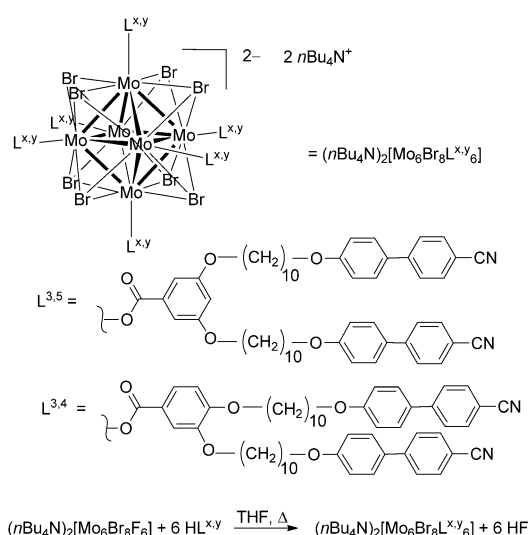
Scheme 1. Representation of (n\text{Bu}_4\text{N})_2[\text{Mo}_6\text{Br}_8\text{L}^{x,y}] .
