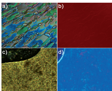
Figure 3. Polarized optical micrographs of a,b) E44/ (n\text{Bu}_4\text{N})_2[\text{Mo}_6\text{Br}_8\text{L}_6^{3,5}] (9:1) mixtures under white light (a) and UV irradiation (b, \lambda_{\text{exc}} = 400 \text{ nm} ), and c,d) E44/ (n\text{Bu}_4\text{N})_2[\text{Mo}_6\text{Br}_8\text{L}_6^{3,4}] (9:1) mixtures under white light (c) and UV irradiation (d, \lambda_{\text{exc}} = 400 \text{ nm} ).
