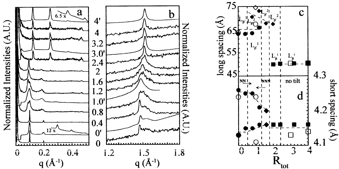
FIGURE 2 SAXS (a) and WAXS (b) patterns at 25°C for different DPPC-enflurane mixtures. The R_{tot} are indicated at the level of each trace: the superscript prime identifies traces measured on D43 line ([lip] = 61 mM). The others are those measured on D22 line ([lip] = 100 mM). Traces 0' and 4' are scale-expanded to make visible the higher order of Bragg peaks. (c and d) Long and short spacings as a function of R_{tot} . Unfilled and solid symbols correspond to measurements on D43 and D22 lines, respectively. (Circles, diamonds, and squares stand for L_{\beta}^{1111} , L_{\beta}^{2111} , and L_{\beta}^i phases, respectively.)
