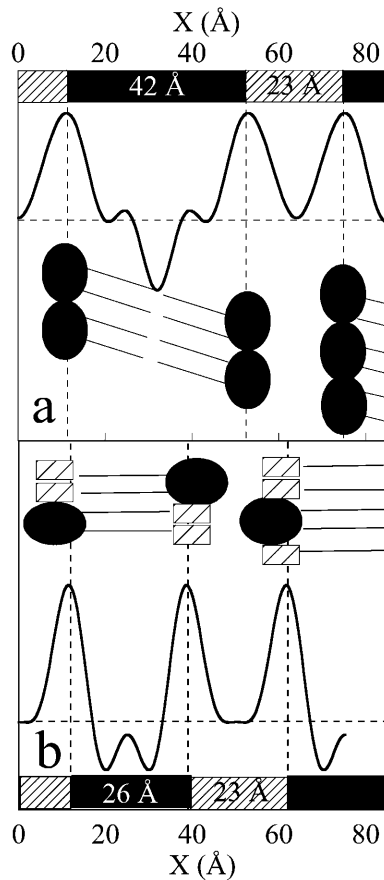
FIGURE 3 Electron profiles calculated from the SAXS patterns of DPPC and Enf-DPPC (0' and 4' traces of Fig. 2). Electron profile of pure L_{\alpha}^1 DPPC lamellar phase (a) and of Enf-DPPC lamellar phase (b). A schematic representation of the lipid organization is also drawn on each panel. These schemes take into account the tilt orientation deduced from the WAXS patterns. The enflurane molecules are represented by a hatched box.
