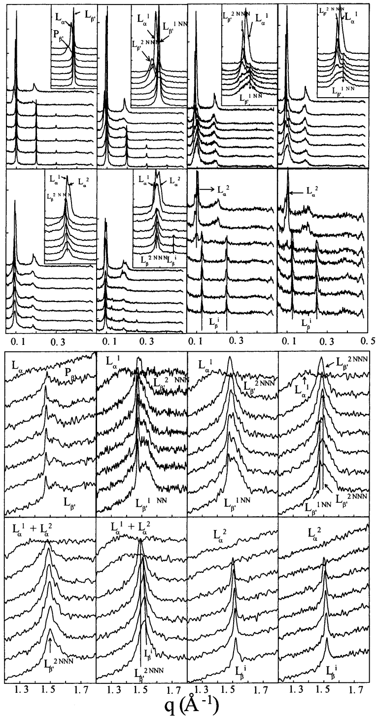
FIGURE 6 SAXS ( upper panels ) and WAXS ( lower panels ) patterns of different enflurane/DPPC mixtures at different R_{tot} and temperatures. In both groups of panels, from left to right and top to bottom, the R_{tot} of the samples are 0, 0.4, 0.8, 1.2, 1.6, 2, 2.4, and 3.2. In each set of traces, the curves, from bottom to top, correspond to measurements at 15, 20, 25, 30, 35, 40, and 45°C. In some cases, inserts present a zoom on the first order of the Bragg peak to evidence coexistence of different lamellar structures.
