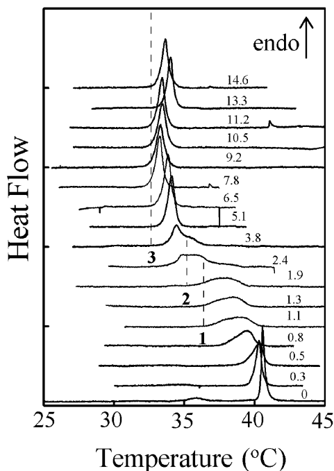
FIGURE 1 Calorimetric curves of pure DPPC multilayers (lower trace) and of different enflurane/DPPC mixtures ( [Lip]_{tot} = 20.3 mM). The R_{tot} are indicated on each curve. The dashed lines 1, 2, and 3 indicate the isothermal event detected on the calorimetric curves.
