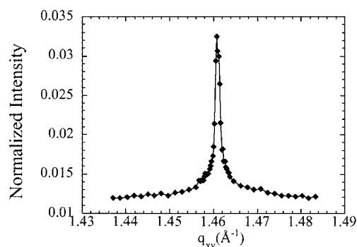
Figure 6. Diffraction pattern of a monolayer of (±)2C16 at T = 41 °C. The peak maximum is at q_{xy} = 1.461 Å −1 , and the full width at half-maximum corresponds to a coherence of a few micrometers.
