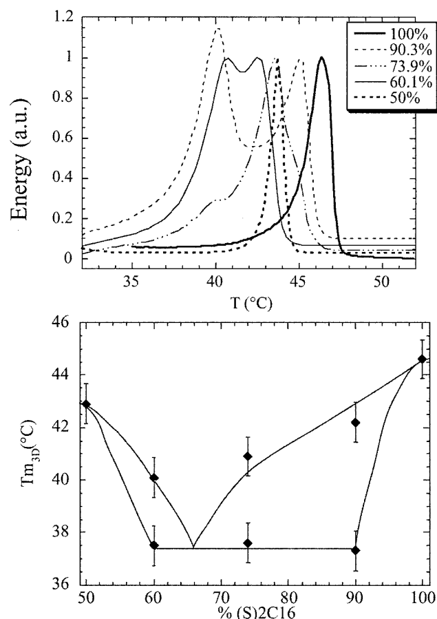
Figure 2. (a) DSC spectra of mixtures of 2-hexadecanol (2C16). The concentration of (S)2C16 within the sample is reported in the inset. (b) Phase diagram (melting temperature vs ratio of both enantiomers) of bulk 2C16. Lines do not correspond to any calculations.
