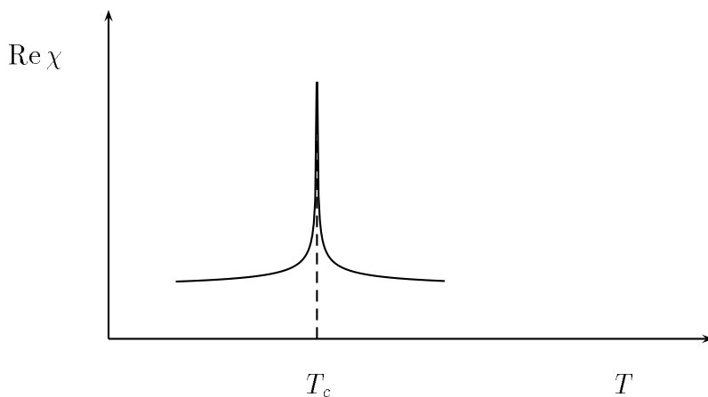
Figure 1: Qualitative behaviour of the real part of the magnetic susceptibility \text{Re } \chi , as a function of temperature T . A cusp-like singularity is observed for T_c .
