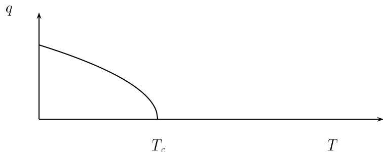
Figure 2: Qualitative behaviour of the order parameter q , as a function of temperature T . An infinite slope singularity is observed for T_c .
