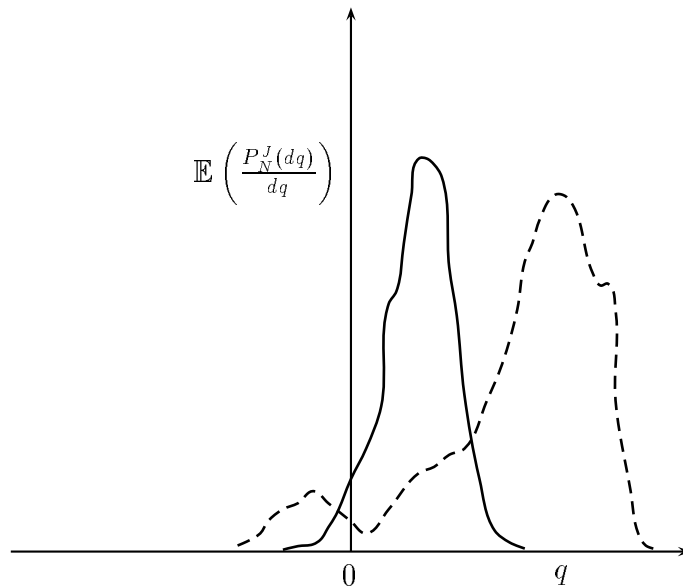
Figure 4: This figure represents the averaged over the randomness probability density for q . The solid line represents the high temperature ( T > 1 ) distribution and the dashed one the low temperature ( T < 1 ) distribution. The results are from [22] and correspond to several hundreds of hours of computer time of Monte Carlo simulations on a finite systems supposed to be so large that the thermodynamic limit is attained. What is meant by ‘large’ depends on the computer budget your laboratory disposes and in the present case it means exactly a box of 15 \times 15 \times 15 sites. We remark that the high temperature distribution is — quite astonishingly — not symmetric around 0 and that the low temperature one develops a small but strictly positive density in the negative axis. This may be due to the small size of the system that feels the boundary condition. In spite of the enormous amount of computer time needed to produce such a figure, in contrast to similar simulations on deterministic systems, it only qualitatively suggests that there is a phase transition.
