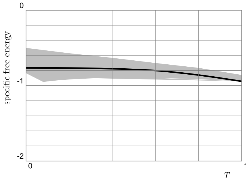
Figure 3: The solid curve represents the value of the specific free energy of the Sherrington-Kirkpatrick model, as predicted by the one replica symmetry breaking computation of [109], as a function of the temperature T , for the low temperature regime T < 1 . The gray region delimits the region where the specific free energy can lie, provided it exists, and it is computed from the rigorous upper bound for \limsup_N f_N of [1] and one of the infinite family of rigorous lower bounds for \liminf_N f_N of [83] best at very low temperature and the rigorous bound of [31] best at intermediate temperatures. No optimisation over the known bounds is performed neither any use of convexity properties is made to delimit the gray area.
