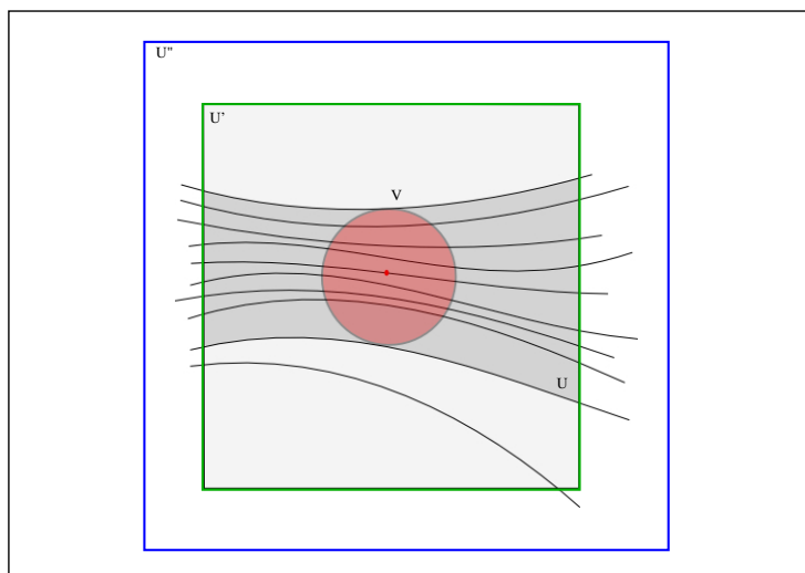
FIGURE 1. The point x is the red point right in the middle of the picture. The open set \mathcal{V} is the red shaded ball, the open set U is grey; U' is light grey with a green contour, and U'' is white with a blue contour. The horizontal curves represent pieces of unstable manifolds (one of them is not a graph above \mathbb{D} ).
