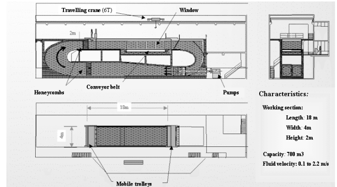
Figure 1. Ifremer free surface hydrodynamic water tunnel.
