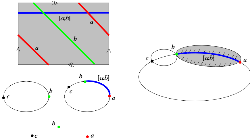
Figure 2.2: A topological resolution tower for \dot{V} .
