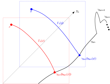
Fig. 15.3. The connecting path \Gamma(x)
