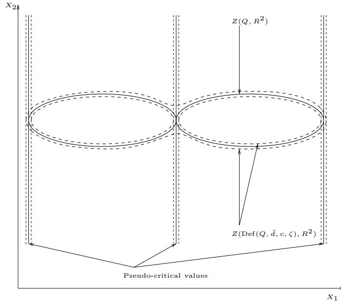
Fig. 12.4. Pseudo-critical values of an algebraic set in \mathbb{R}^2
