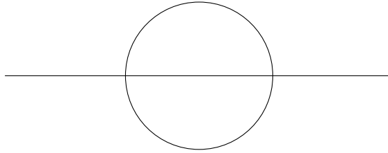
Fig. 11.1. \text{Zer}(P_1, \mathbb{R}^2) and \text{Zer}(P_2, \mathbb{R}^2)
