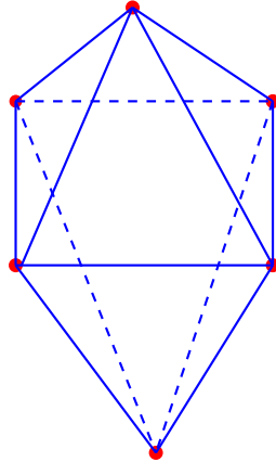
Fig. 5.3. A two dimensional simplicial complex homeomorphic to S^2
