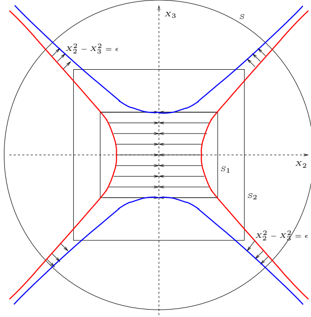
Fig. 7.4. S_1 and S_2
