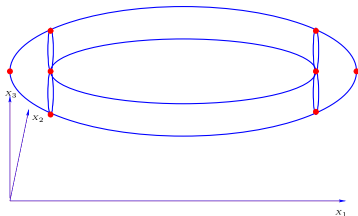
Fig. 15.2. The roadmap of the torus
