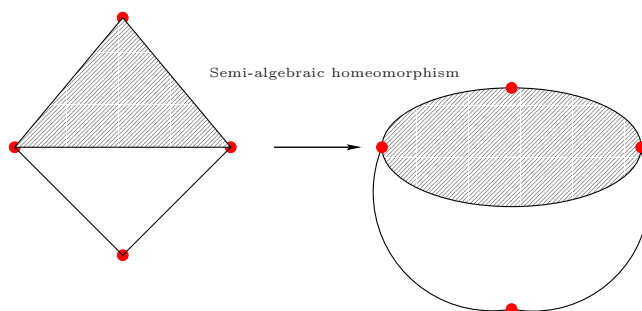
Fig. 5.5. Semi-algebraic triangulation
