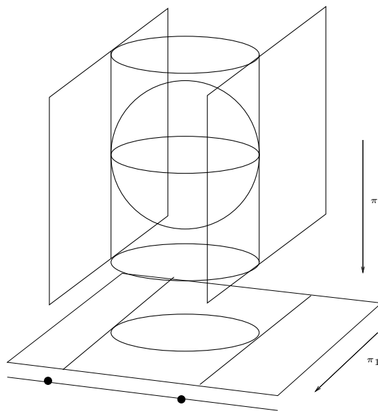
Fig. 5.1. A cylindrical decomposition adapted to the sphere in \mathbb{R}^3
