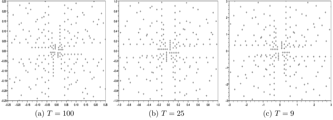
Figure 2: The ‘scaling property’. For \Gamma = \text{SL}(2, \mathbf{Z}) , parts of the orbit of three different points are shown, at different scales and with different values of T . Each contains approximately 200 points.
