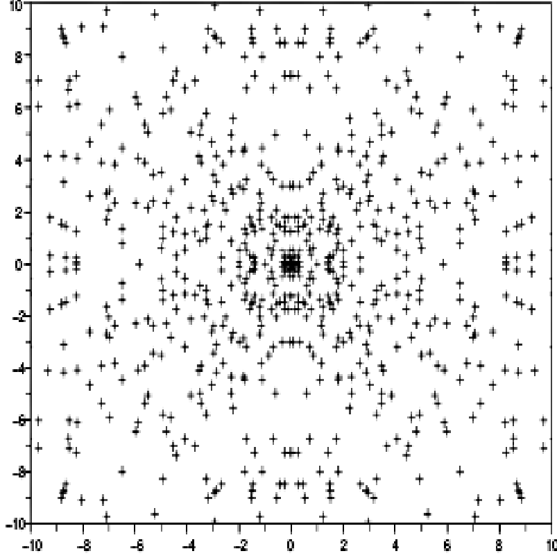
Figure 1: ‘Cloud’ for the cocompact lattice \mathrm{SL}_1(D_{2,3}(\mathbf{Z})) , \mathbf{u} = (1, 0) , T = 100 .
