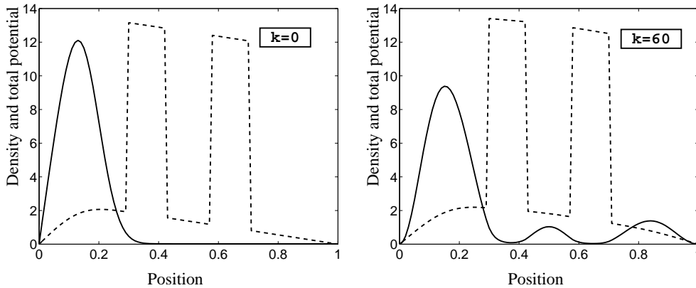
Figure 1. Left: Initial density n(x) (solid line) and corresponding total potential (V + V^{ext})(x) (dashed line). Right: density and potential after 60 iterations.
