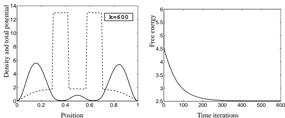
Figure 2. Left: density n(x) (solid line) and total potential (V + V^{ext})(x) (dashed line) after 600 iterations. Right: Evolution of the free energy S^k .
